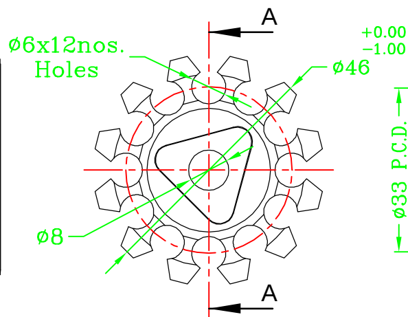
BOBBIN Ø46MM
