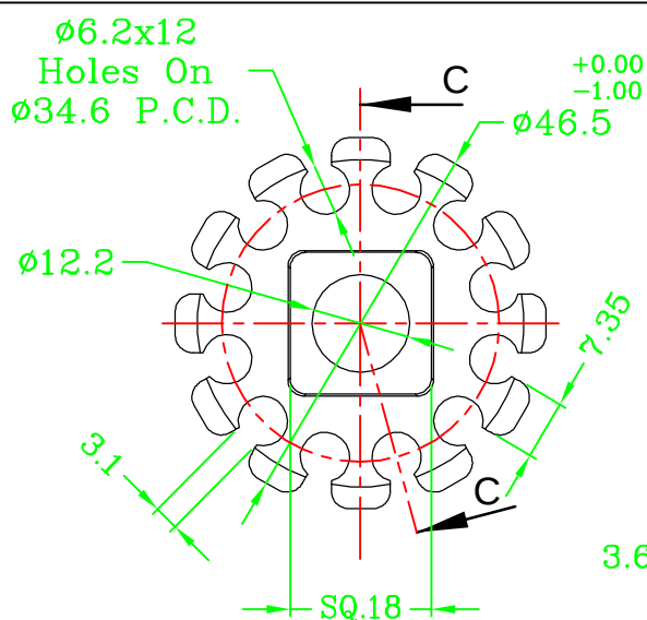
BOBBIN Ø47MM
