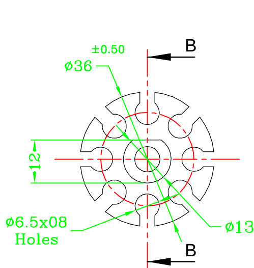
BOBBIN Ø36MM
