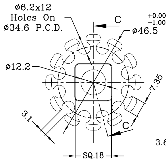
BOBBIN Ø47MM
