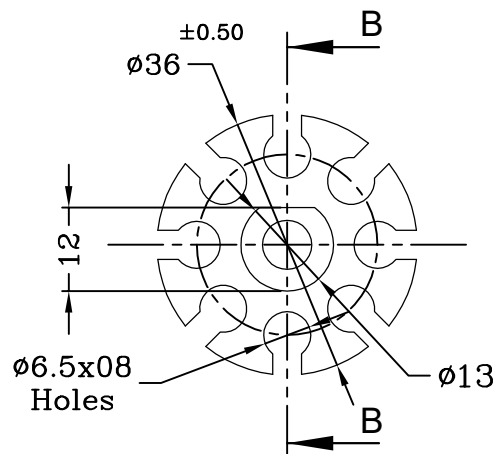
BOBBIN Ø36MM
