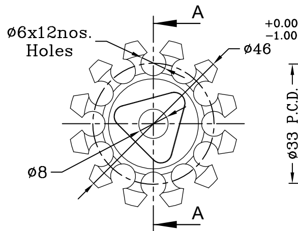
BOBBIN Ø46MM
